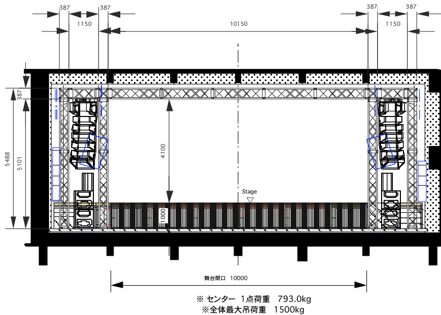
Front View 1Truss~2Truss
